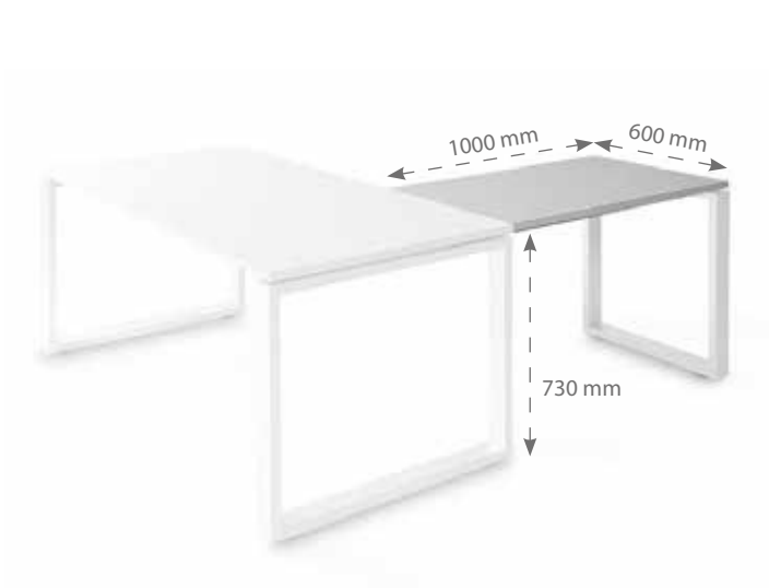
● SKA5092-BL-BL / 1000x600
